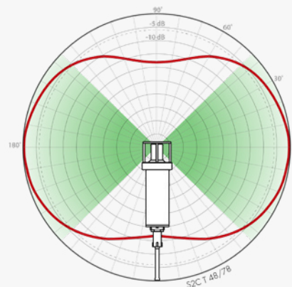
Transducer directivity pattern
